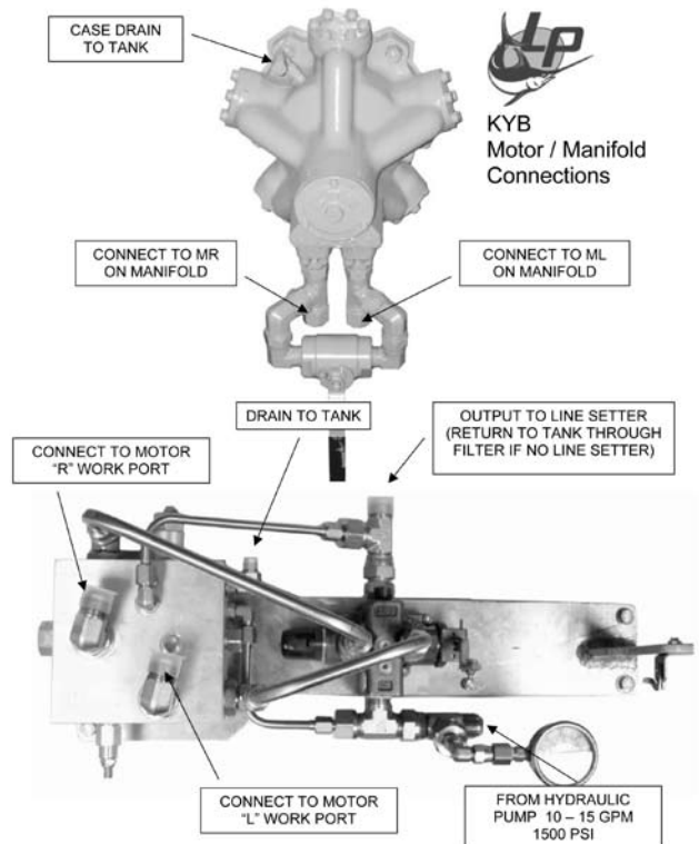
40" Diameter Reels w/ KYB Motor
