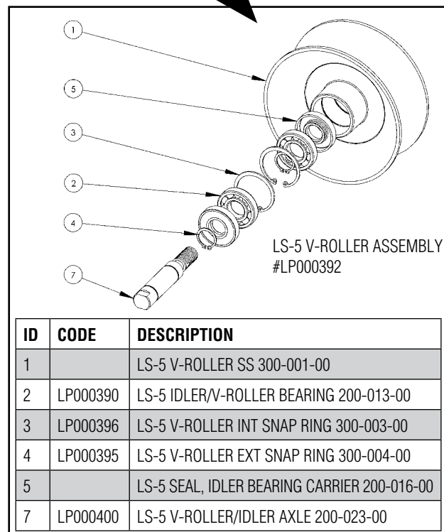
V-Roller Detail
