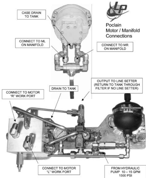
48" Diameter Reels w/ Poclain Motor
