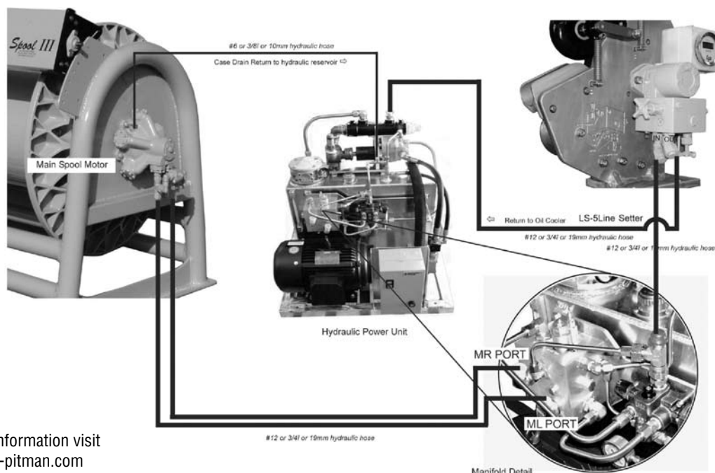
LP SUPER SPOOL III HYDRAULIC CIRCUIT CONNECTIONS
