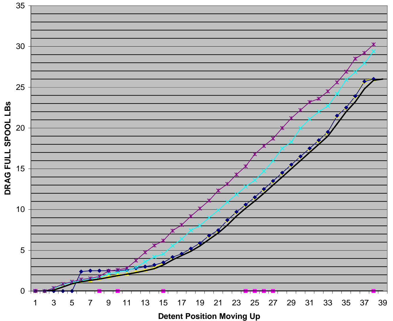
SERIES A ANDROS 5II DRAG CURVE Reworked CAM (-.020" Detent 0-14) J. Nomura Jan 11, 2015
